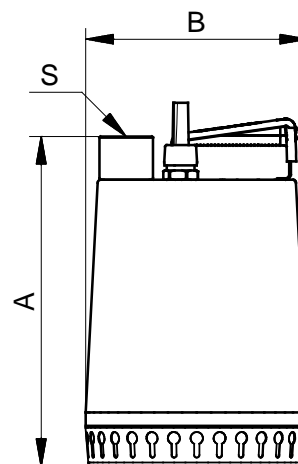
Fig. 16 Pump dimensions
