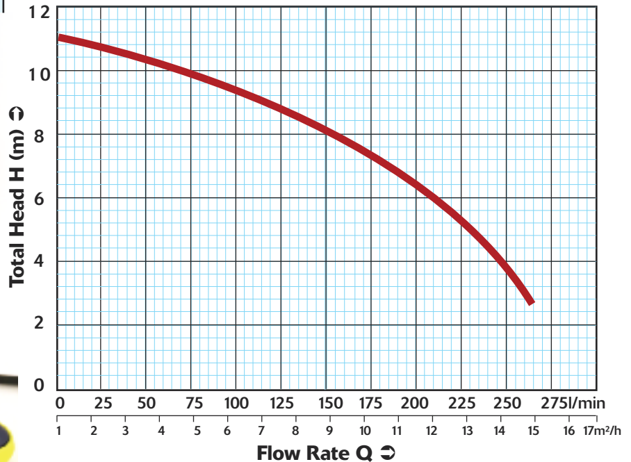
PERFORMANCE CHART AT n = 2860 r/min
